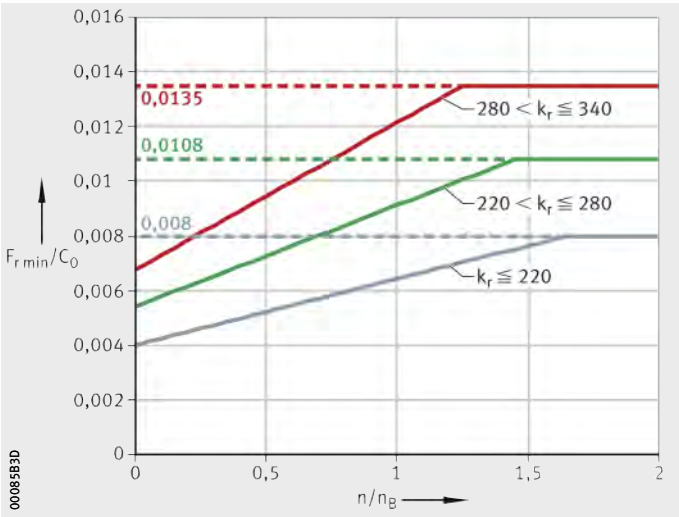
Figure 9 Minimum load with oil lubrication
