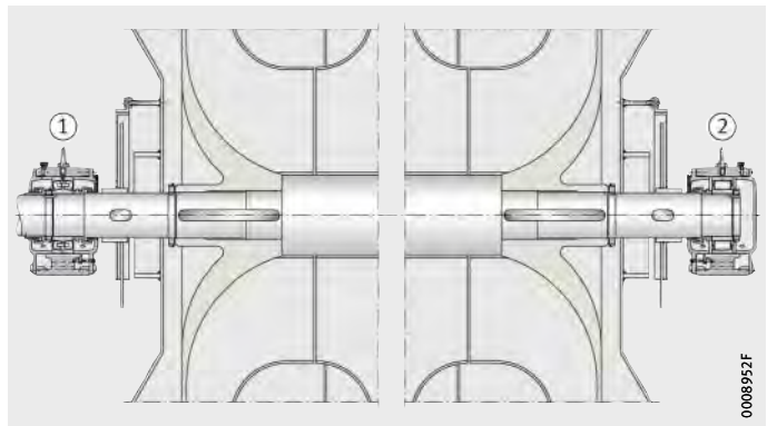
Figure 2 Blower bearing arrangement
